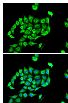
Fig. 2. Immunofluorescence analysis of A-549 cells using CPT1A antibody. Blue: DAPI for nuclear staining.
