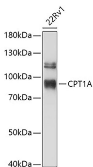
Fig. 1. Western blot analysis of extracts of 22Rv1 cells, using CPT1A antibody at 1:1000 dilution. Secondary antibody: HRP-labeled Goat Anti-Rabbit IgG(H+L) (A0208) at 1:1000 dilution. Lysates/proteins: 25µg per lane. Blocking buffer: QuickBlock™ Blocking Buffer (P0231). Detection: BeyoECL Star (P0018A). Exposure time: 1s.
